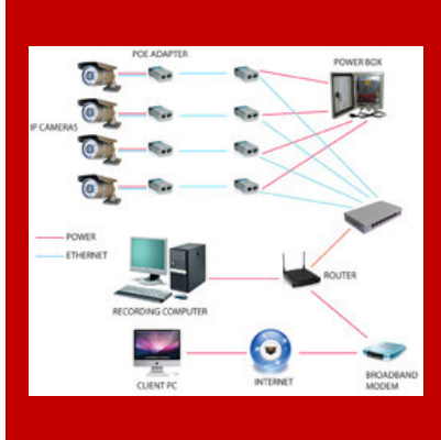
IP CCTV Camera System
